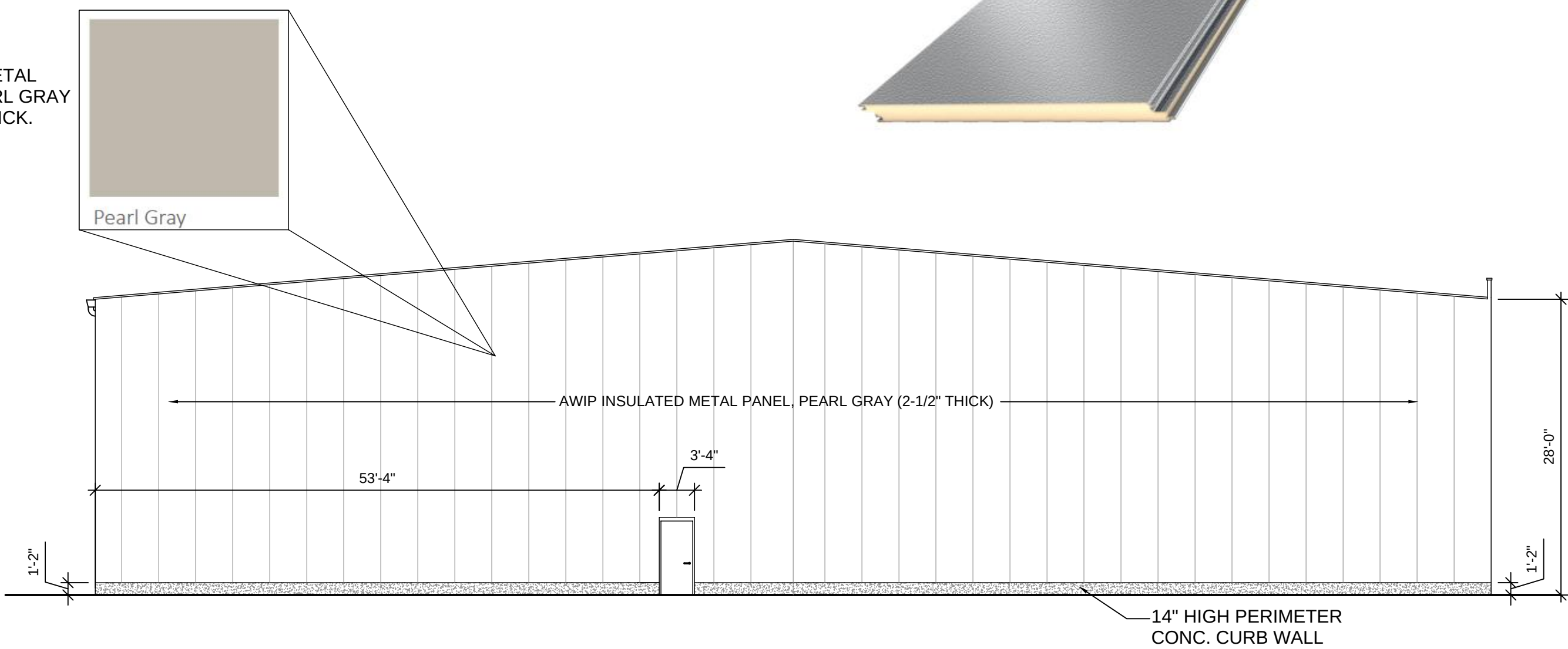
SOUTH ELEVATION
