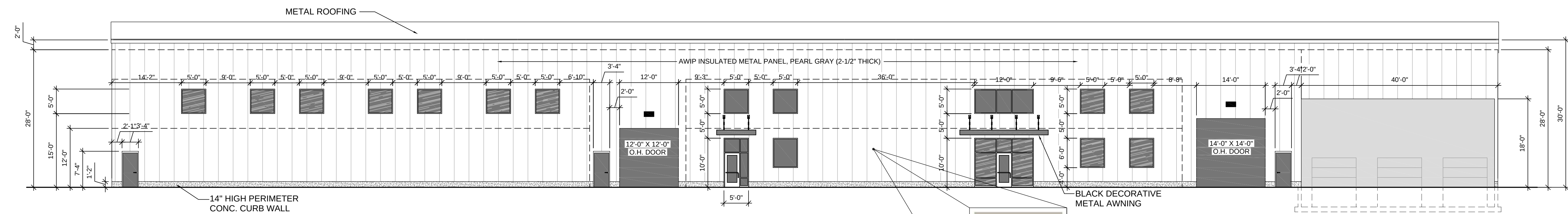
EAST ELEVATION
