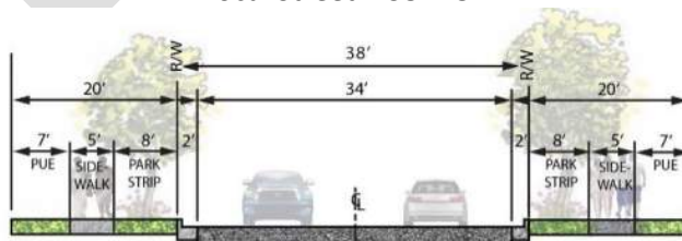
Local Street – 38' ROW
